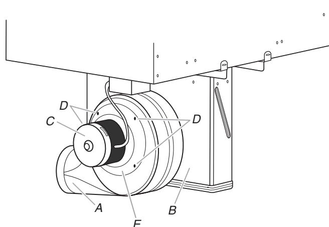
A. Blower exhaust scroll B. Plenum C. Blower motor D. #10-32 locknuts (4) E. Motor mounting plate
