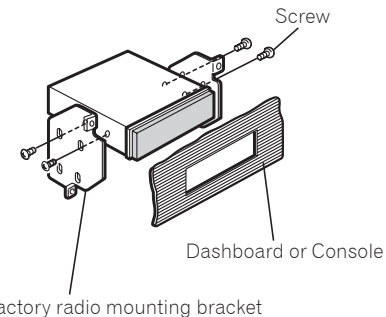
Factory radio mounting bracket
